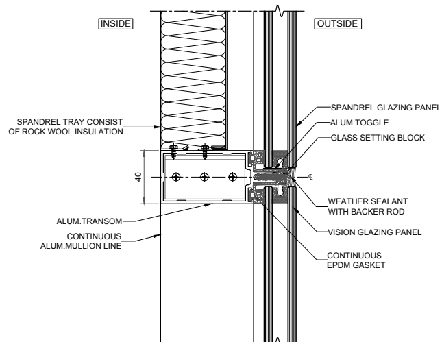
TYPICAL TRANSOM SECTION
